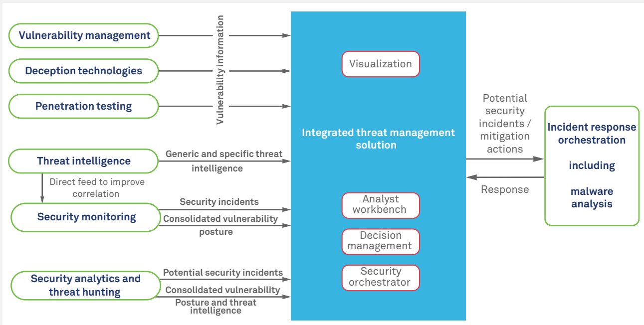
Figure 1: Indicative architecture of the solution
