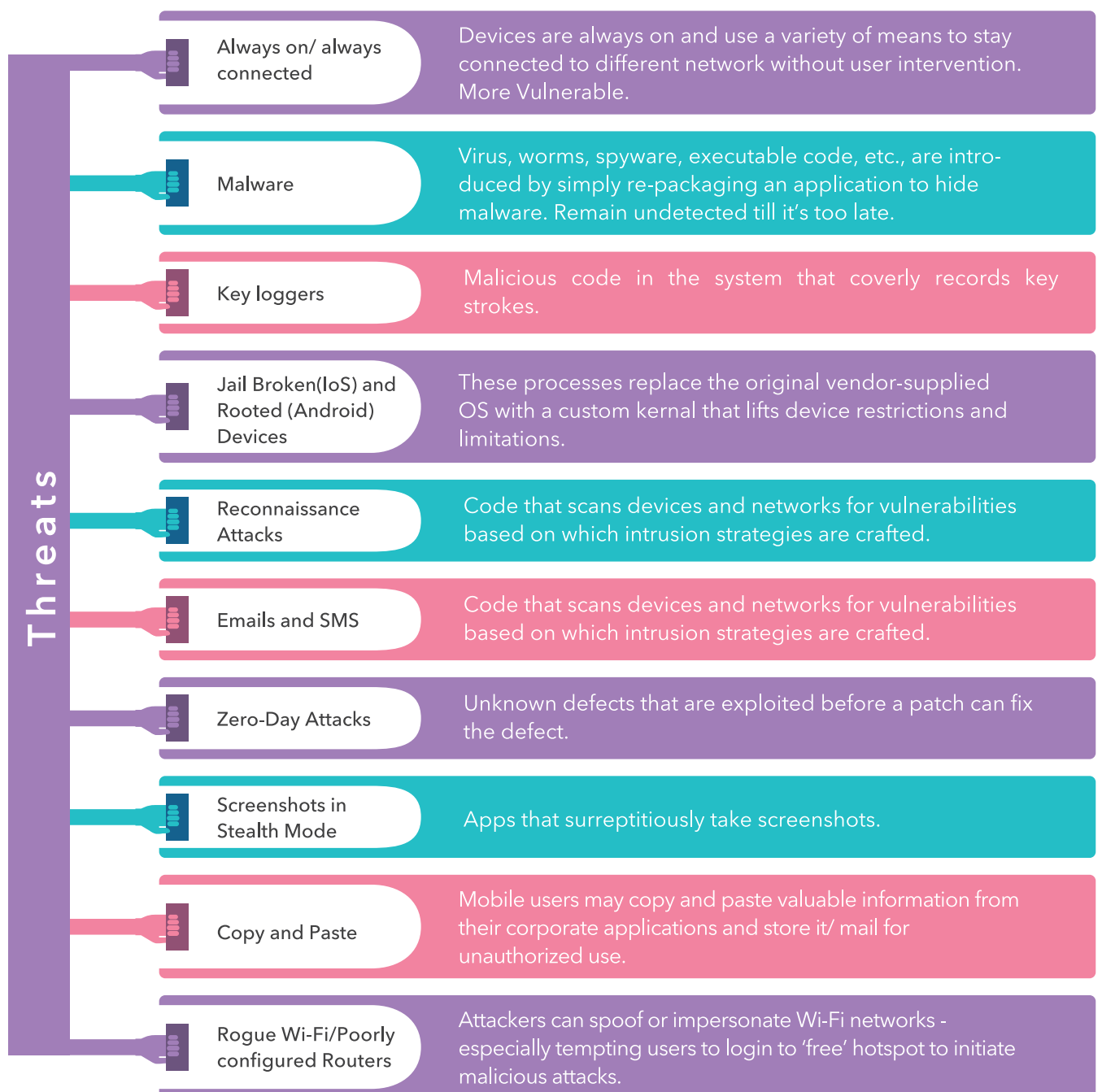
Fig 1: Common Mobile Computing Threats
