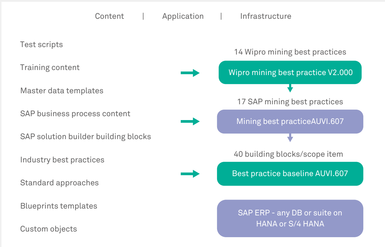
Figure 1: Solution overview
